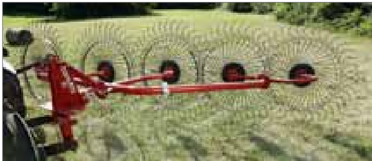
Finger wheels are mounted on oscillating arm
